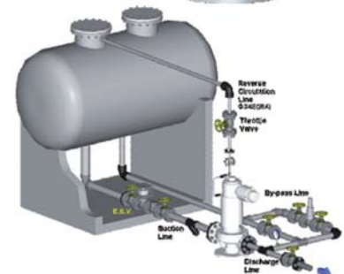
Over Ground In-Line Type
